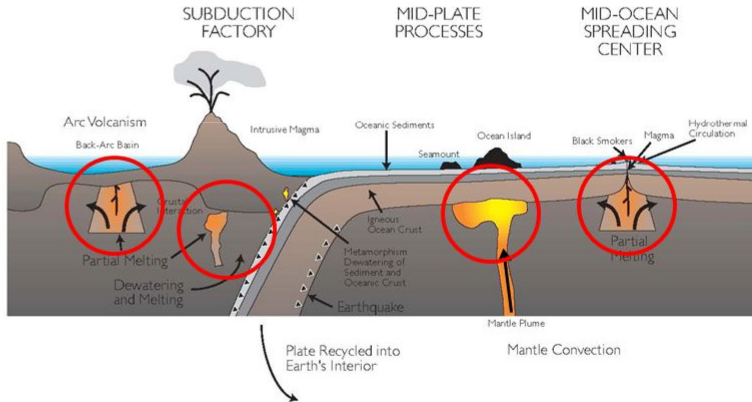
Figure 20. Schematic drawing of the solid Earth's plate tectonics.
